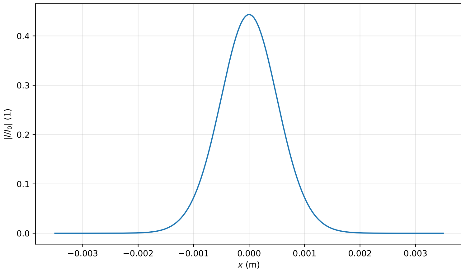
Intensity profile I(x, y = 0, z = 2.627m)/I_0 , P_{in}=0.2P_{cr} , artificial time
